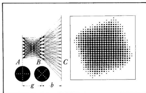
Fig. 2. Apparatus system of Pinhole Structures. Multiple pinhole camera combined with light pattern subject. A: Light pattern subject, variable. B: Multiple pinhole, variable. g: Distance A-B, variable. b: Distance B-C, variable. C: Pinhole Structure, result.
